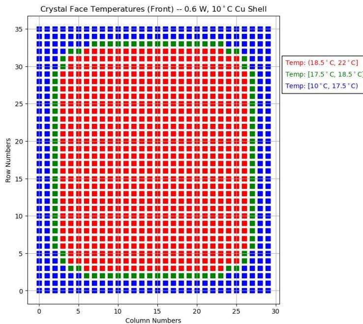
Temperature plot for Q = 0.6 W simulation with 10°C Cu shell
